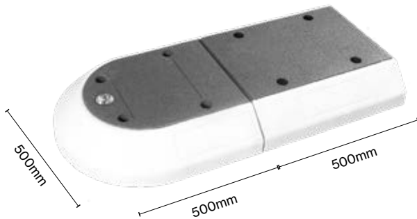
Rubber Cycleway and Traffic Islands are modular allowing you to create sections of any length.
