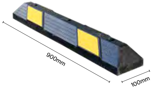
900mm Rubber Wheel Stops are suited for unique situations like asset protection shown here.
