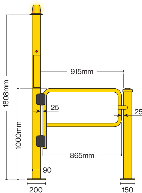
ALERT POST SHOWN WITH 76MM GATE BOLLARD (SOLD SEPARATELY)
